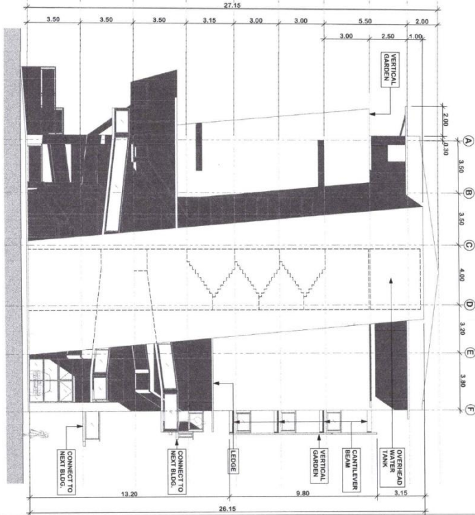
2 RIGHT SIDE ELEVATION 1:100
