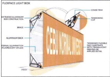
Reference - Panaflex Signage Construction Detail
